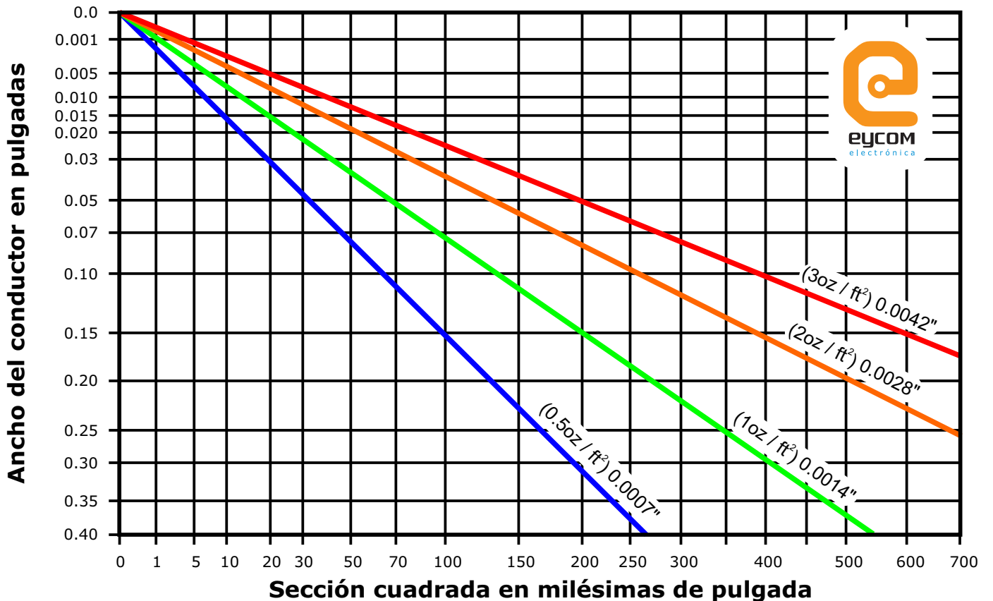
[Fuente: IPC2221 - Generic Standard on Printed Circuit Board Design]
