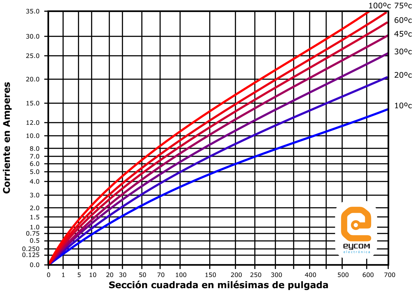
[Fuente: IPC2221 - Generic Standard on Printed Circuit Board Design]
